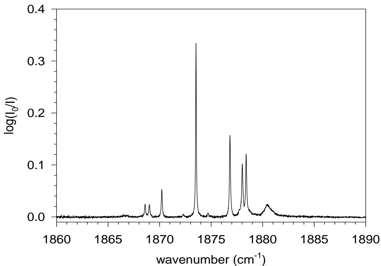
Figure 1: An FTIR spectrum of ^{14}\text{NO} trapped in solid para-hydrogen at 4.3 K.
