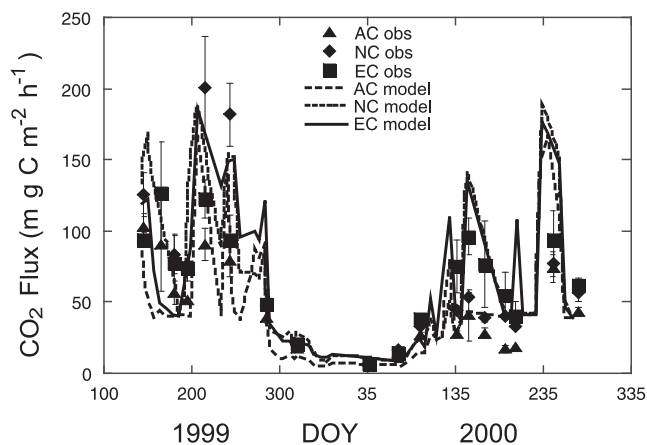
Figure 3. Soil respiration rates modeled by DAYCENT [Parton et al. , 1998; Del Grosso et al. , manuscript in preparation, 2003] (“Model,” lines) compared with measured rates (“Obs,” symbols). Treatments are abbreviated as in Figure 1.
