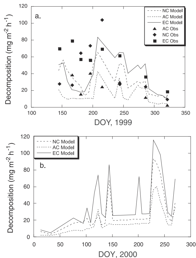
Figure 7. Decomposition rates in two growing seasons. (a) Measured (“Obs,” symbols) and simulated (“Model,” lines) estimates of the decomposition flux for 1999, and (b) simulated estimates for 2000. Measured values were partitioned using ^{13}\text{C} and then normalized to Fallow plot values to include all decomposition components. DAYCENT abiotic decomposition submodel was used for the simulations (Del Grosso et al., manuscript in preparation, 2003).
