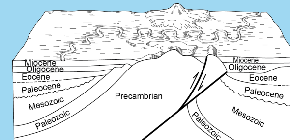
Late Eocene to mid-Miocene (35–11.6 million years ago) erosion and burial of the Laramie Mountains.
