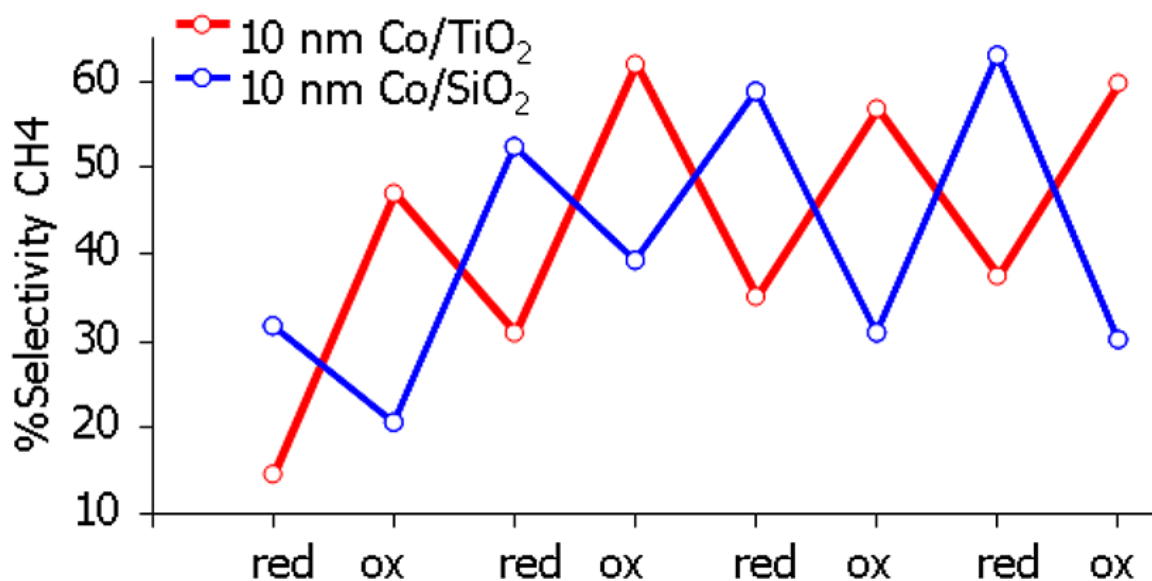
Figure 4. Cobalt catalyst percent selectivity to methane over \text{TiO}_2 and \text{SiO}_2 supports in both reduced and oxidized states.
